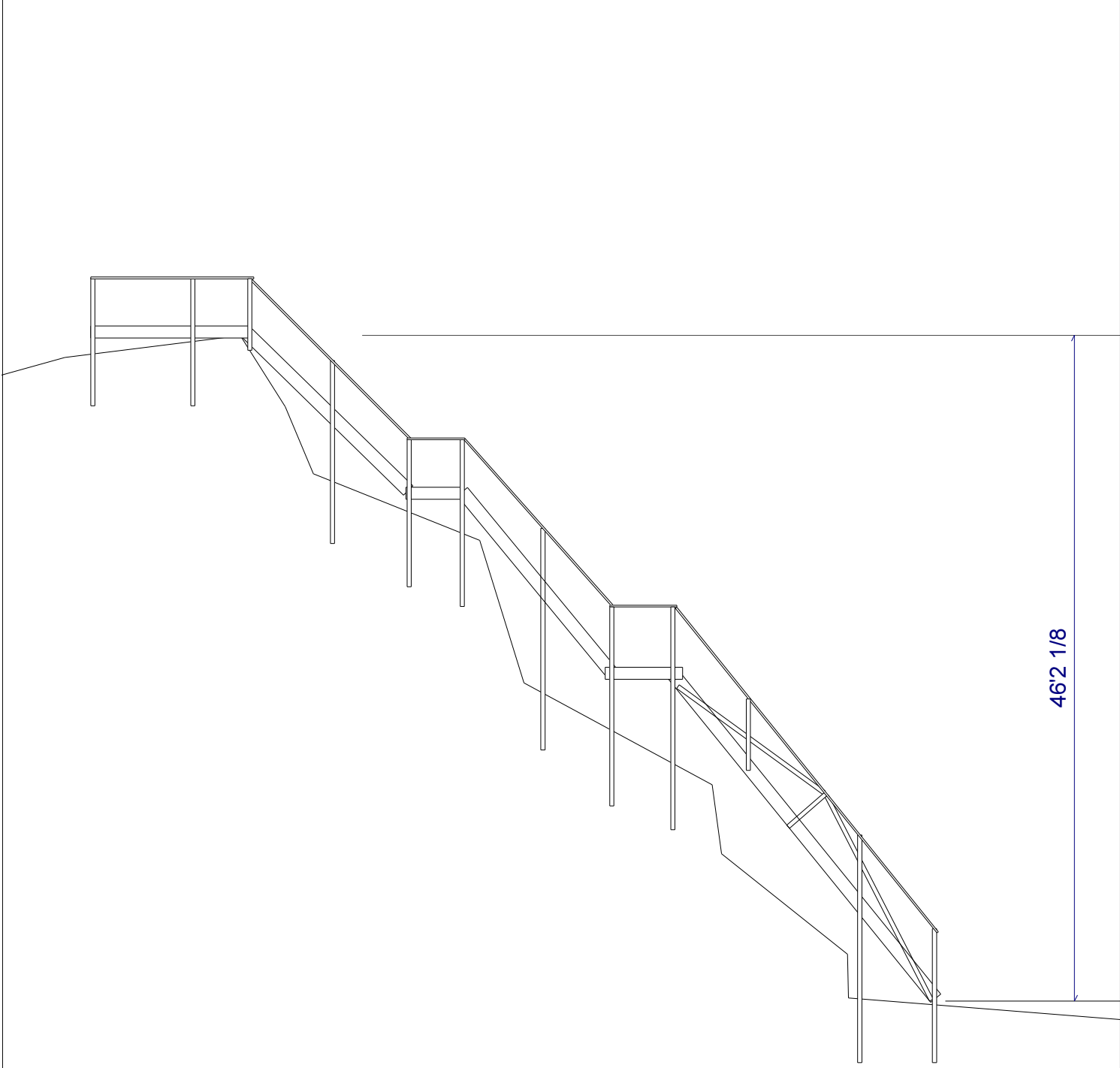
Cross Section - 1" = 10'
