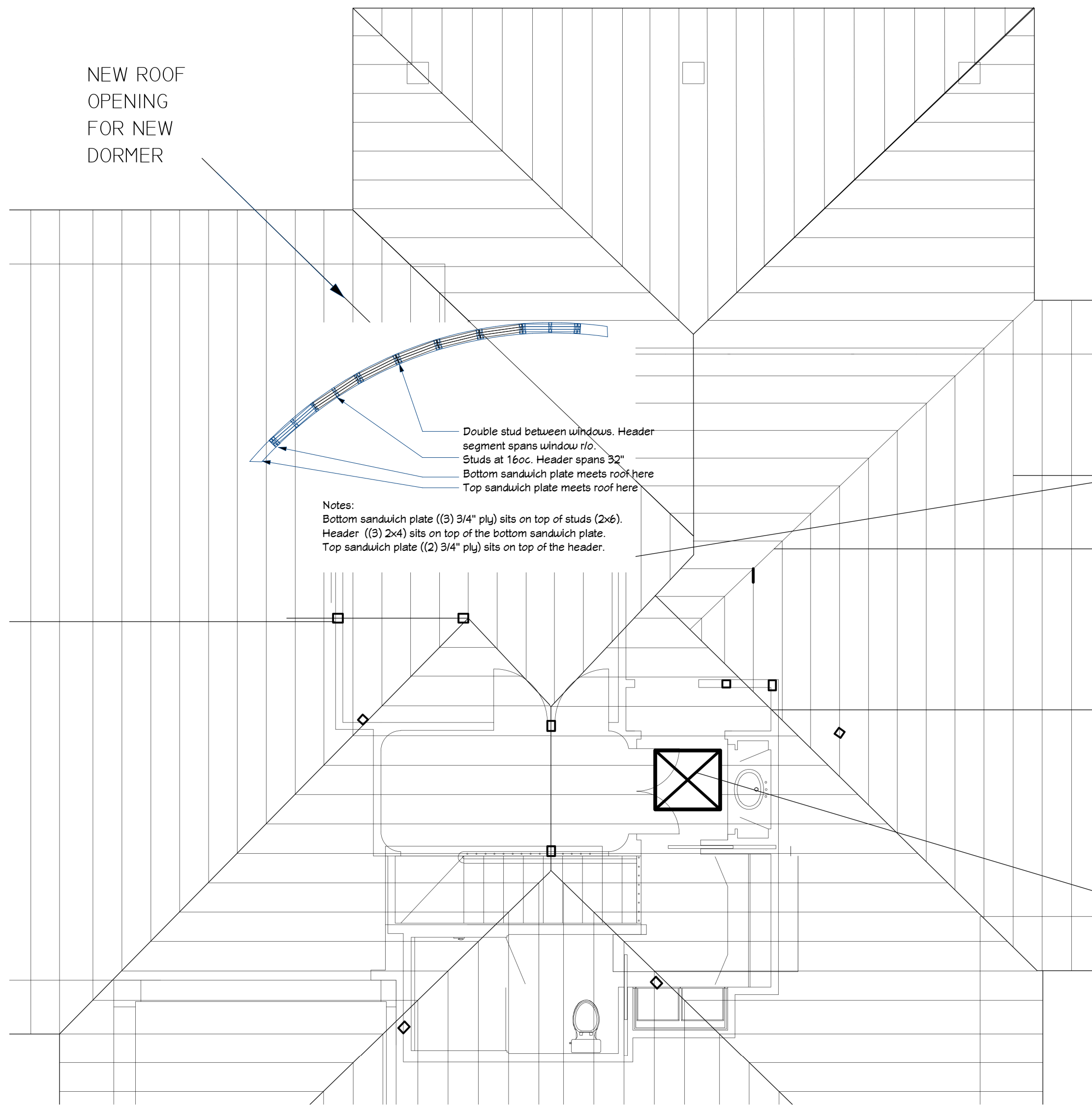
Curved Dormer Wall Detail
