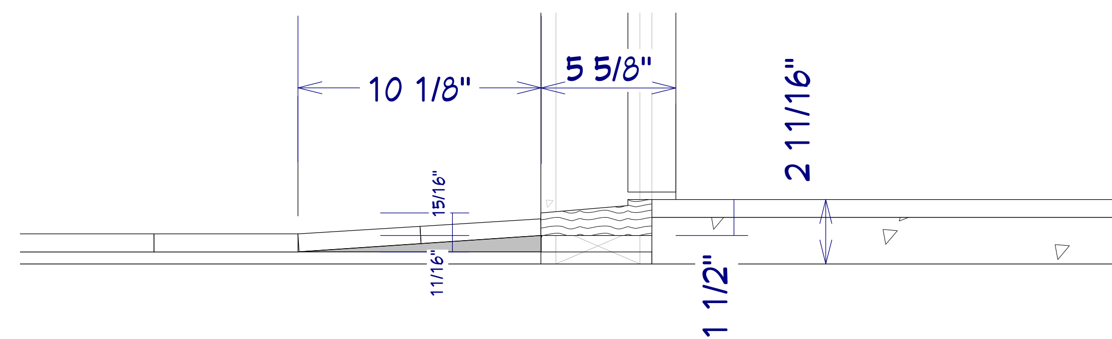
Vanity Ramp
