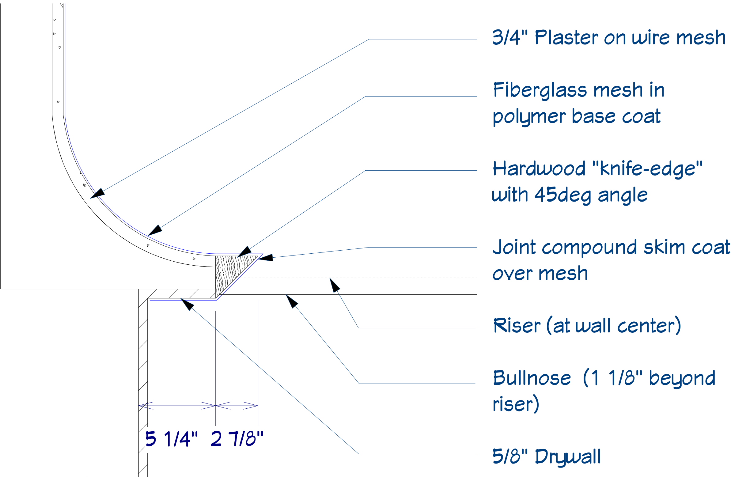
Plan Detail at Top of Stair
