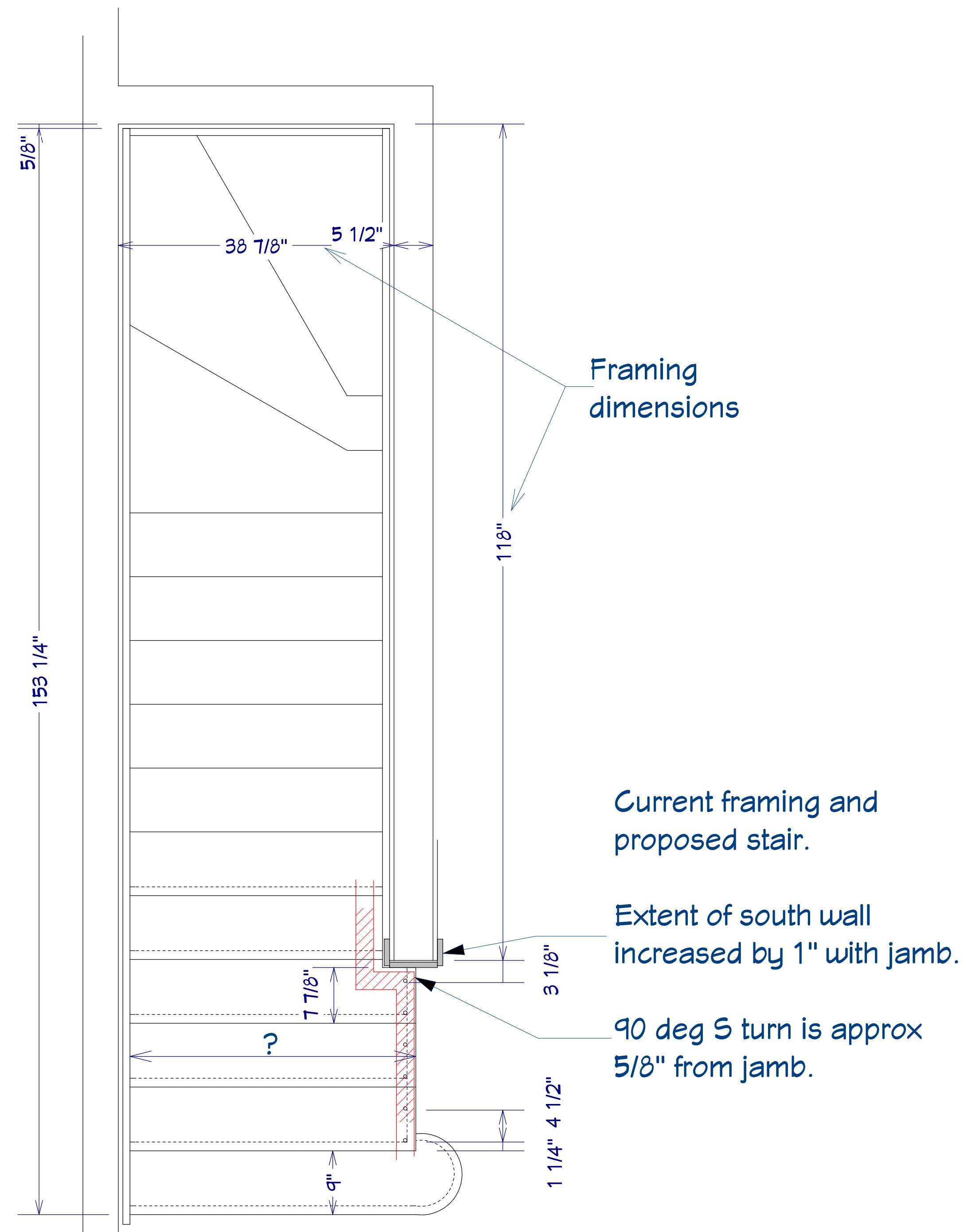
Tread notch and S turn detail
