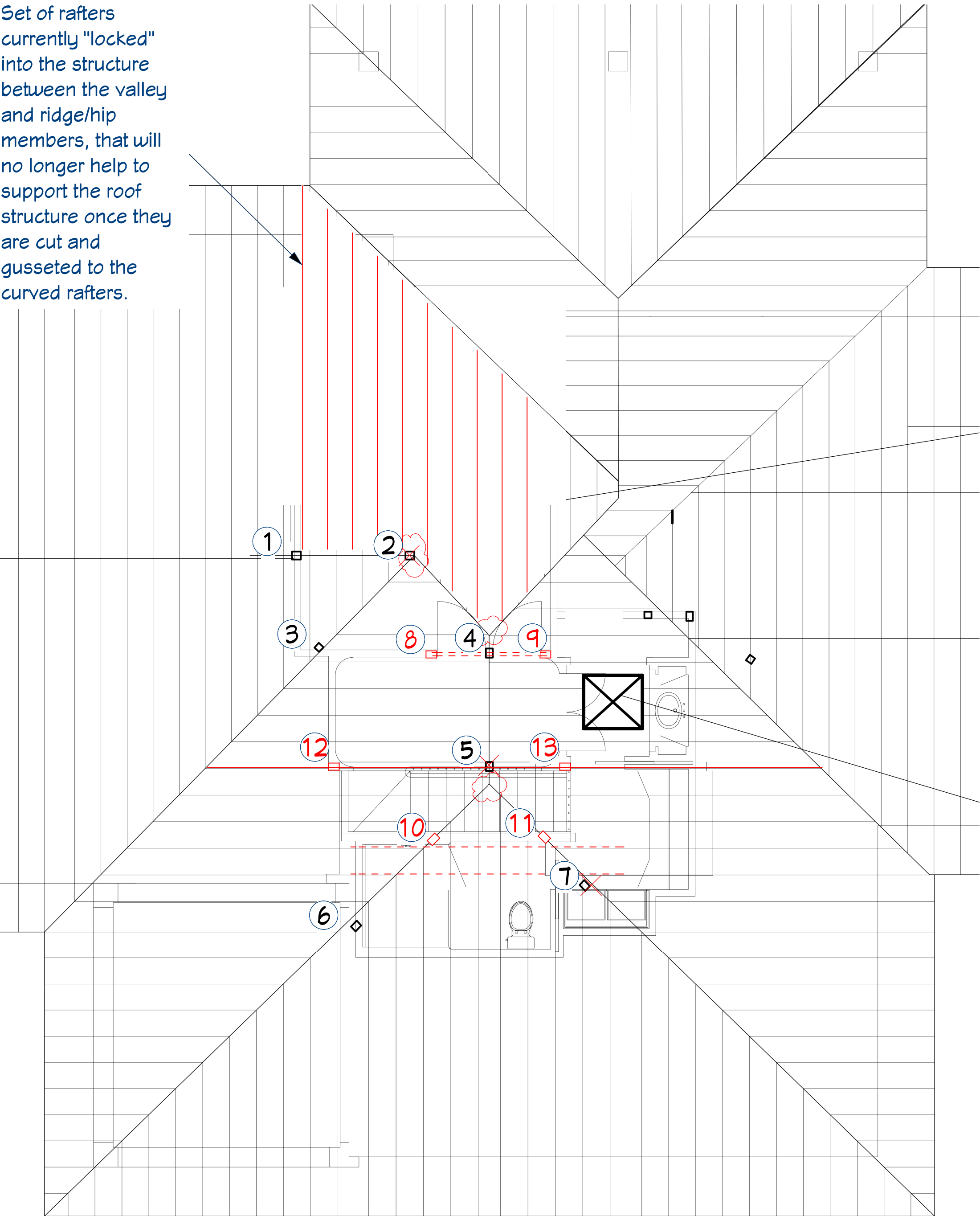
Roof Structural Posts
