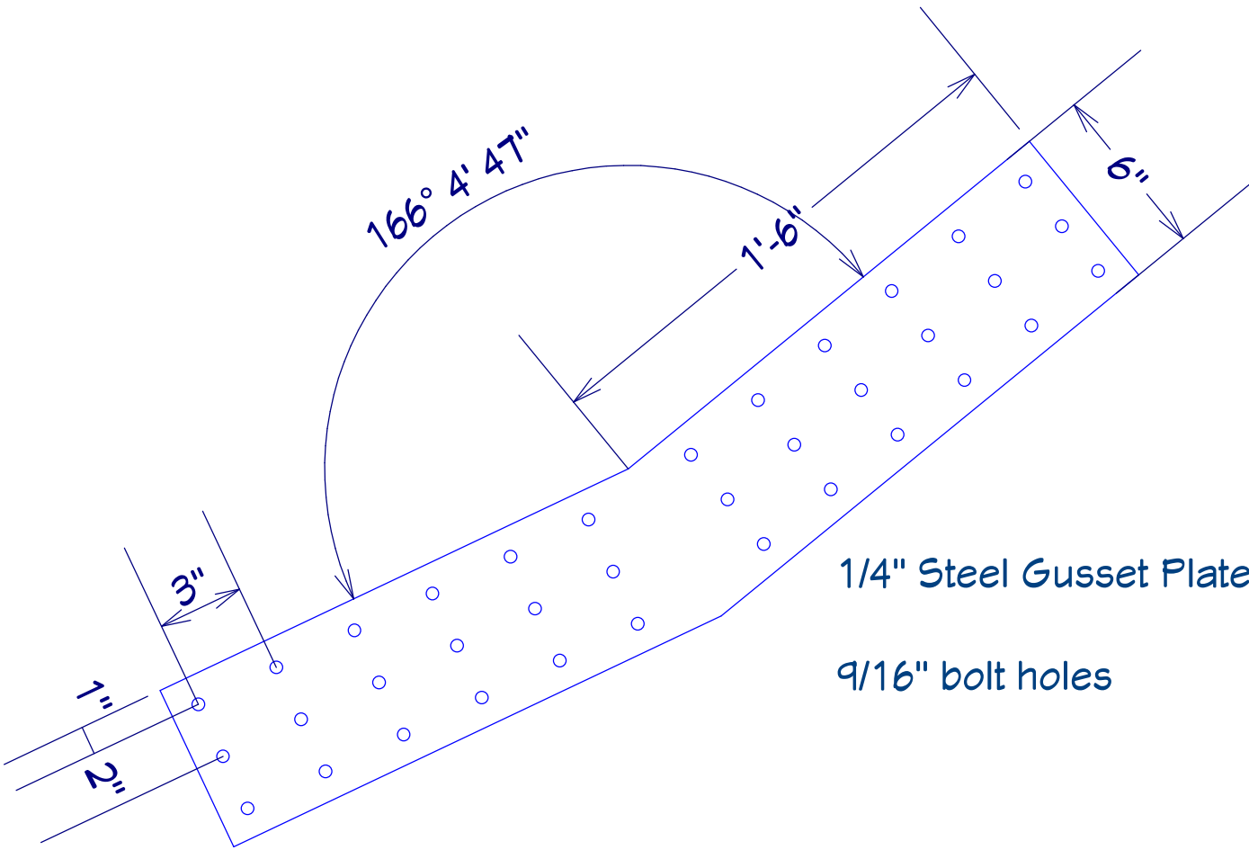
Gusset Pattern 1
