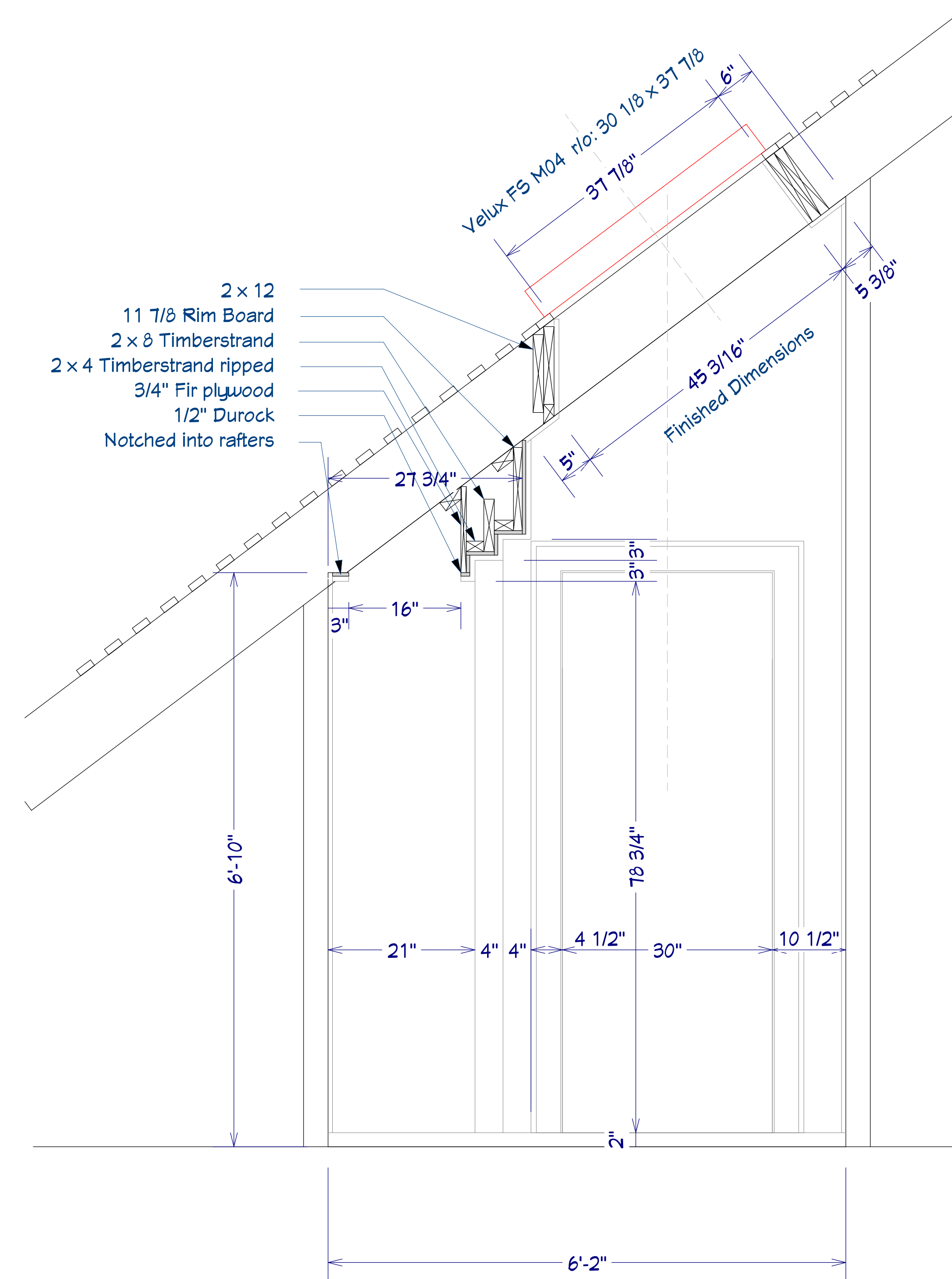
Section at Lavatory
