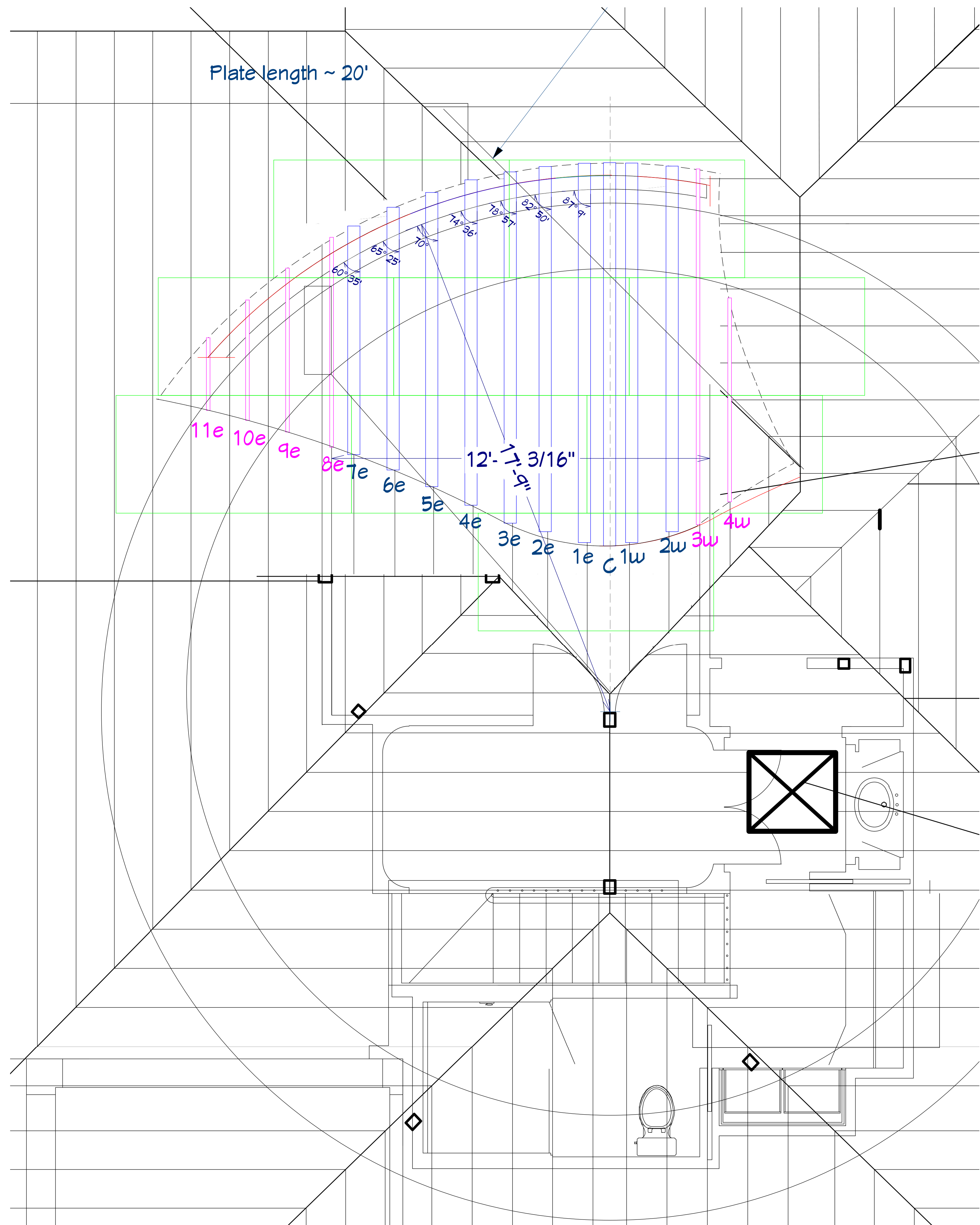
Dormer Rafters
