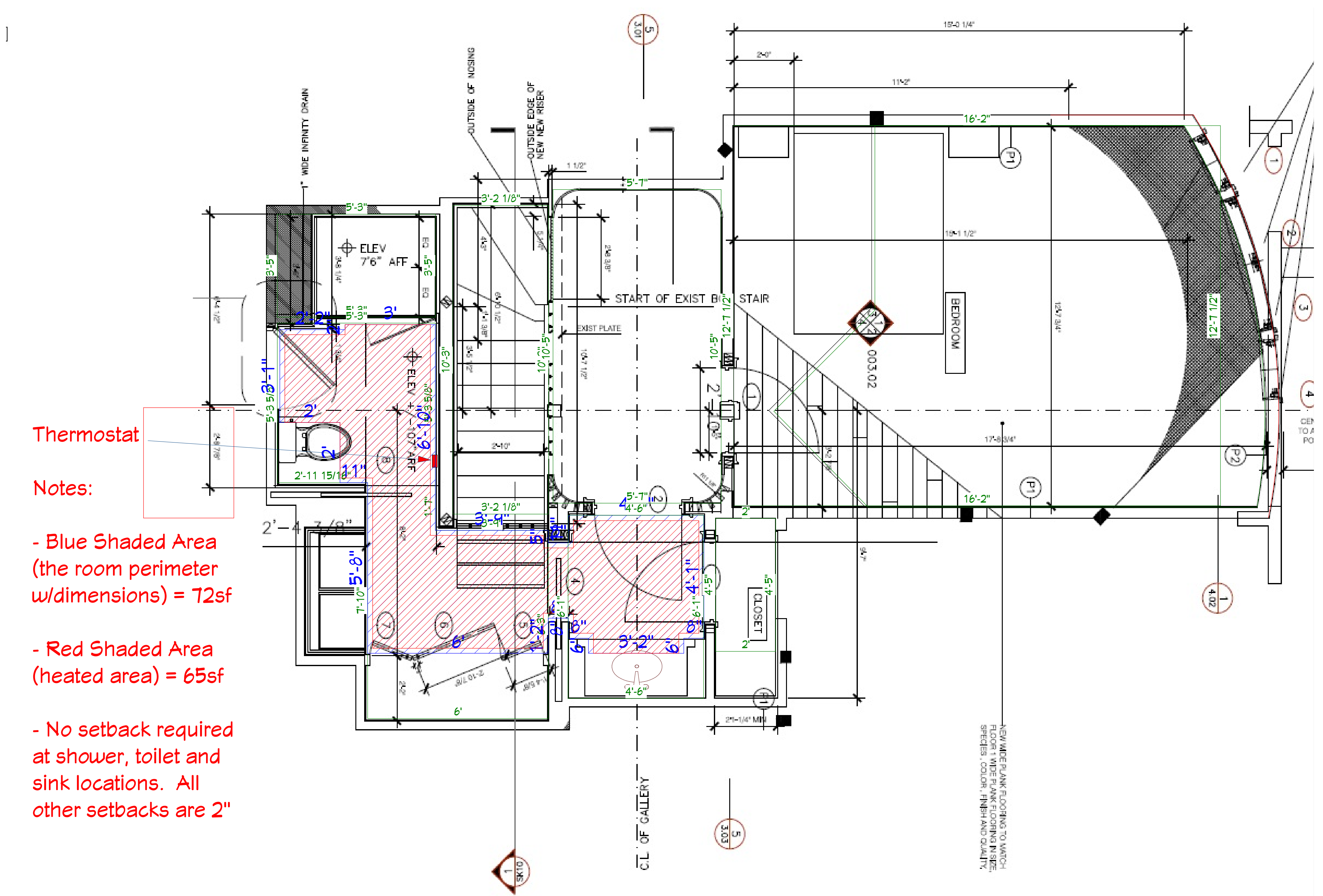
Radiant Heat Area (floor plan by Paul Regan Architect) Scale: 1/2" = 1'
