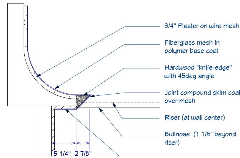
Plywood Shoe dimensions
