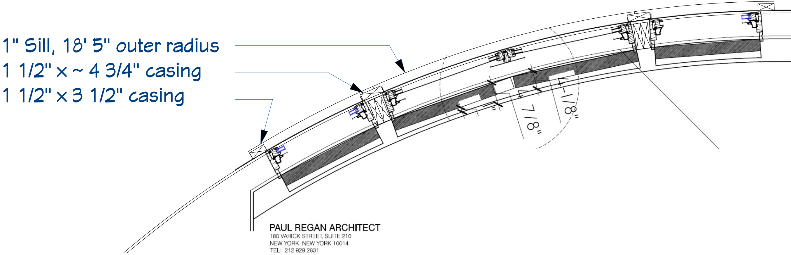
Window Trim Plan (overlaid on drawing by PR) Scale: 1" = 1'
