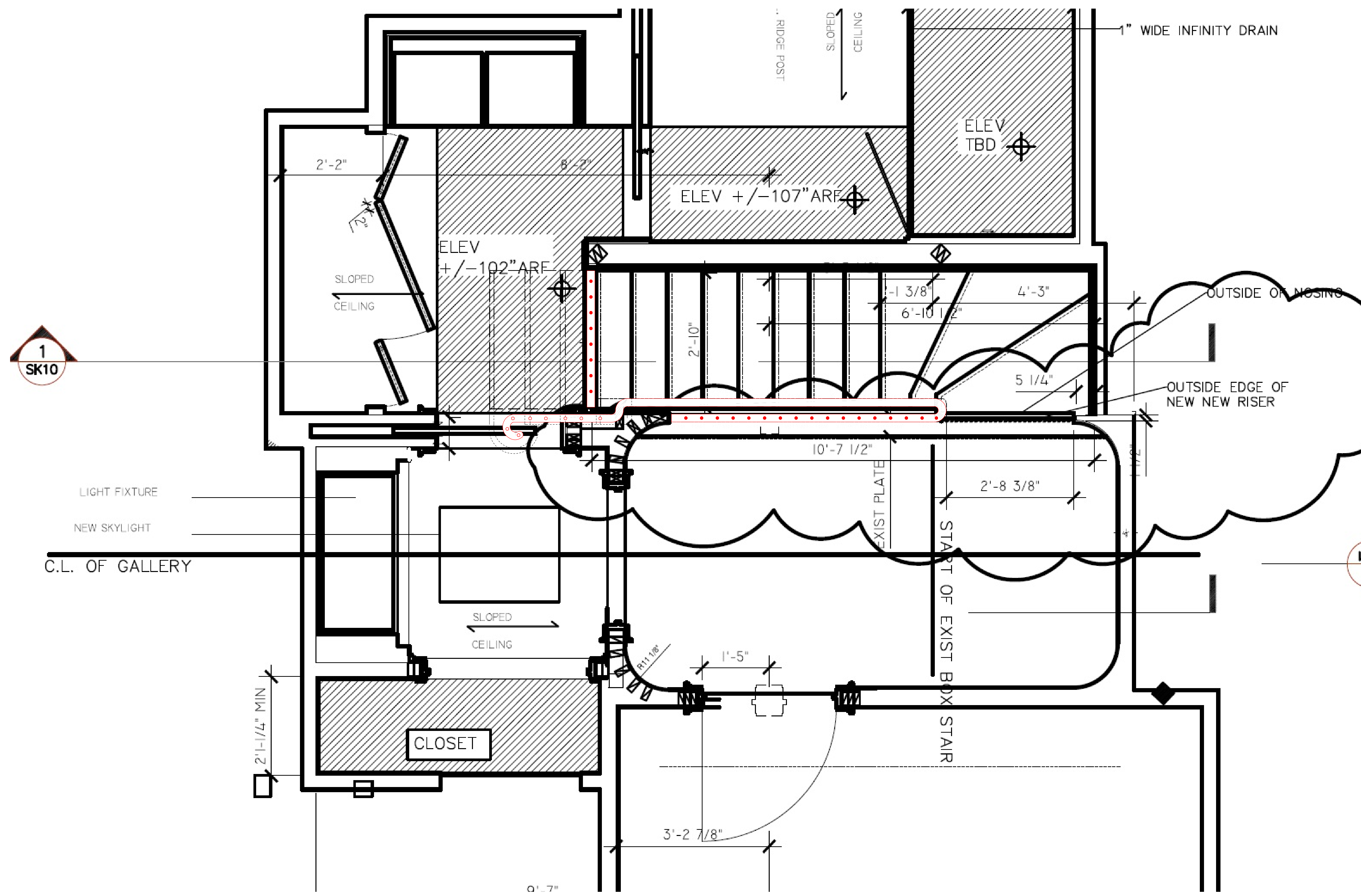
Railing Plan (Overlaid on drawing by Paul Regan, Architect)
